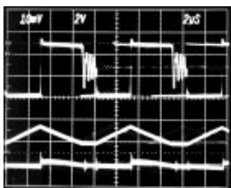
SWITCHING WAVEFORMS— DISCONTINUOUS CONDUCTION
