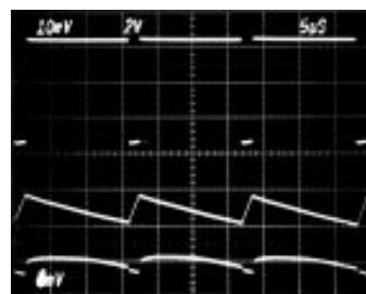
STEP-DOWN CONVERSION
