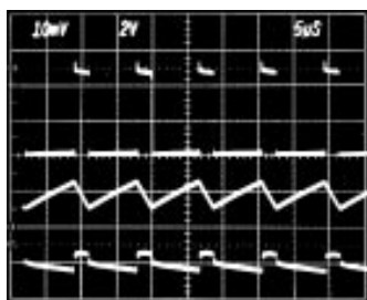
SWITCHING WAVEFORMS— CONTINUOUS CONDUCTION
